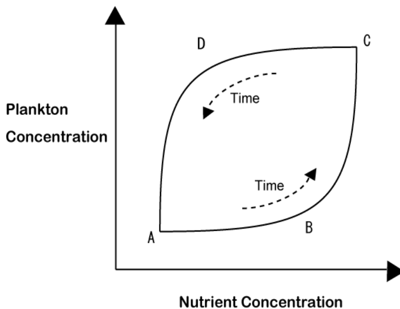
Figure 1. Buffering Capacity of Lakes to Increasing Nutrient Concentrations, Illustrating Non-linear (Hysteresis) Responses to Degradation and Remediation Efforts.
