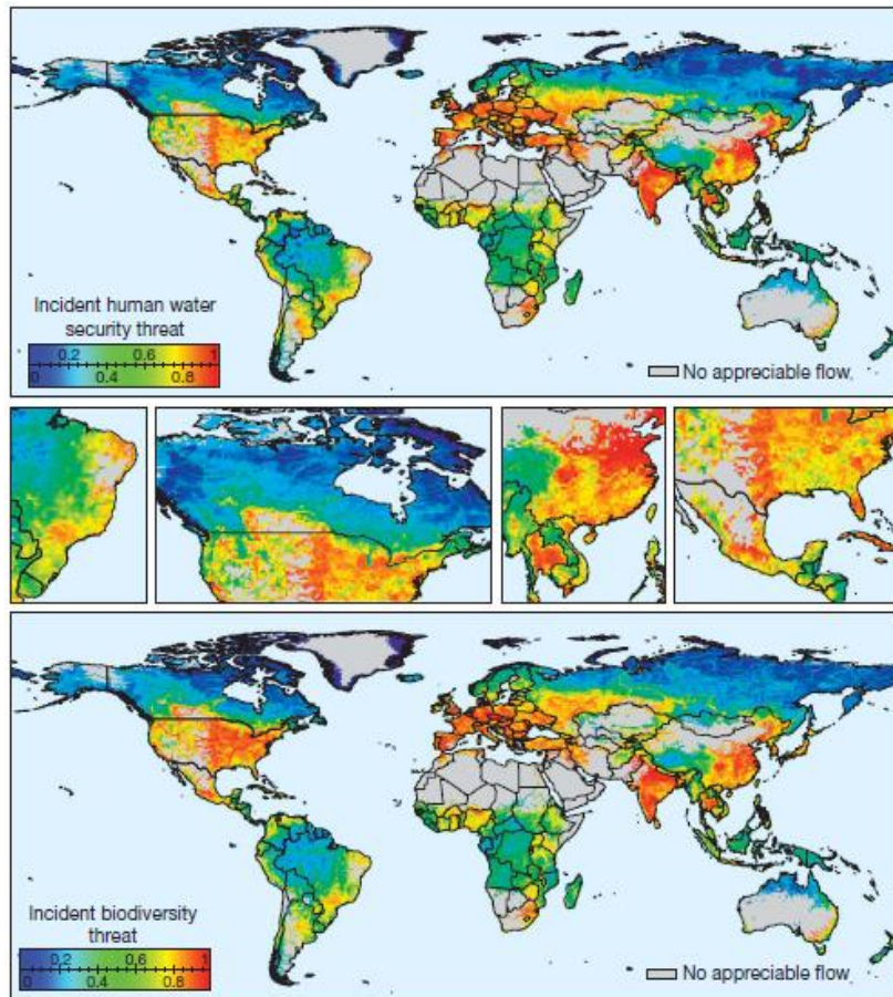
Figure 3. Global Overview of Incident Human Water Security (HWS) and Biodiversity (BD) Threats (Vörösmarty et al. 2010)
